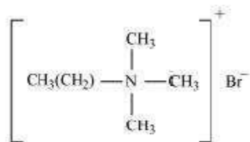
Cetyltrimethylammonium bromide
