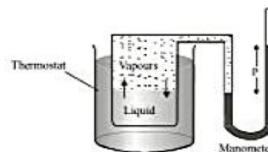
Physical equilibrium between liquid \rightleftharpoons vapours
