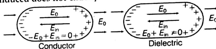
Behaviours of a conductor and a dielectric in an external electric field
