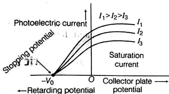
Variation of photoelectric current versus potential for different intensities but constant frequency
