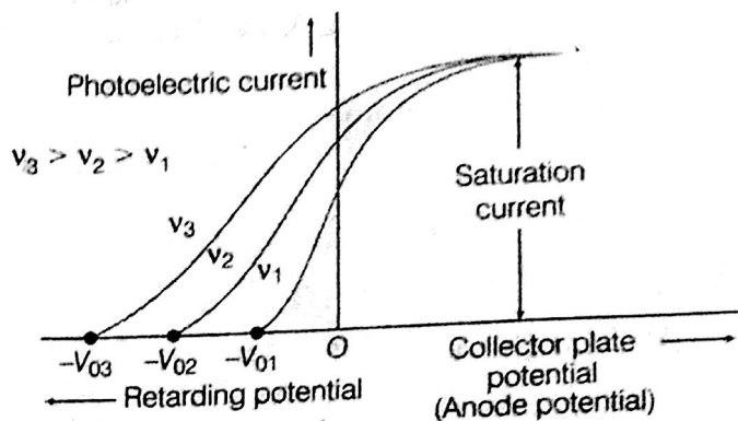
Variation of photoelectric current versus potential for different frequencies but constant intensity of light
