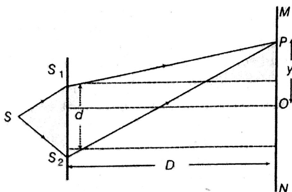
Young's arrangement to produce interference pattern
