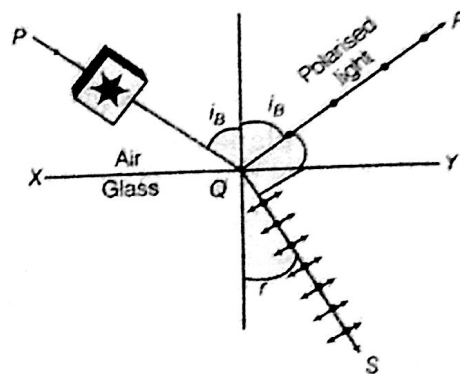
Polarisation by reflection
